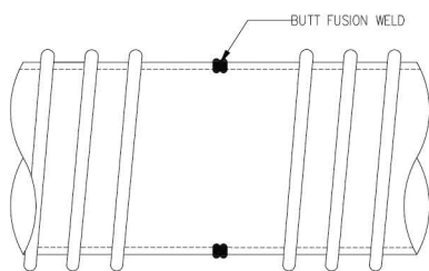
'SPIRAL' BUTT FUSION WELD JOINT
