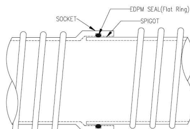
'SPIRAL' RUBBER RING JOINT
