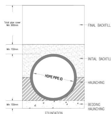
PIPE EMBEDMENT MATERIALS
