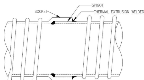
'SPIRAL' THERMAL EXTRUSION WELDED JOINT
