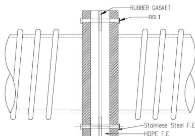
'SPIRAL' BOLTED FLANGE JOINT
