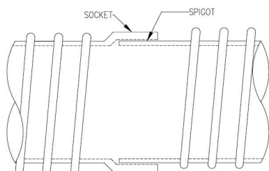
'SPIRAL' SOCKET AND SPIGOT JOINT
